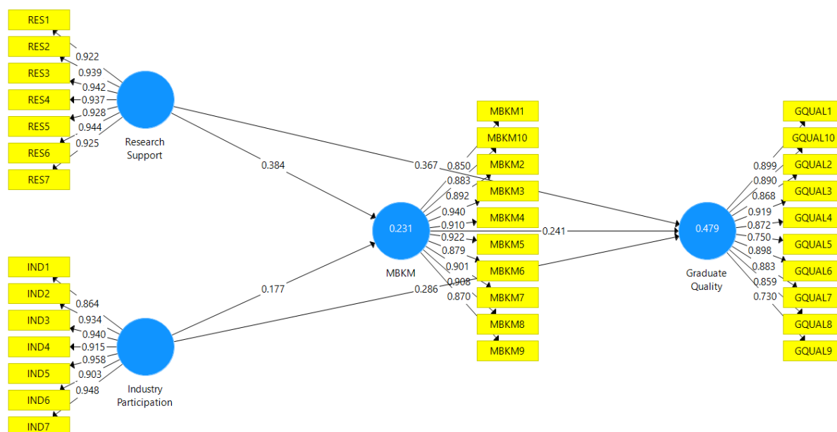
Figure 1 PLS Algorithm
