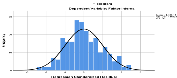
Figure 1 Normality Test
